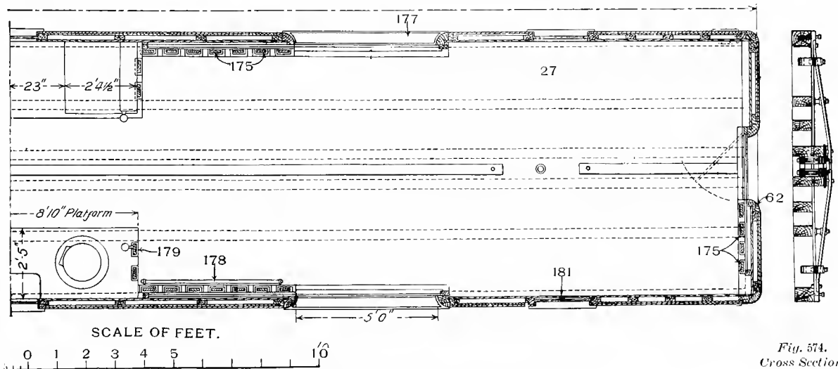
Fig. 573. Half Plan and Horizontal Section of Sides. BAGGAGE AND EXPRESS CAR. BALTIMORE & OHIO RAILROAD.
